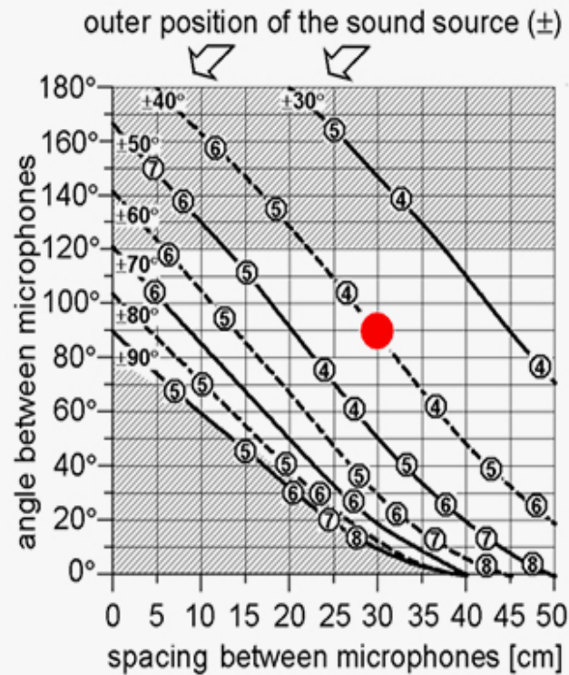
Fig. 24 The DIN setup marked in a general diagram for cardioid microphones.
