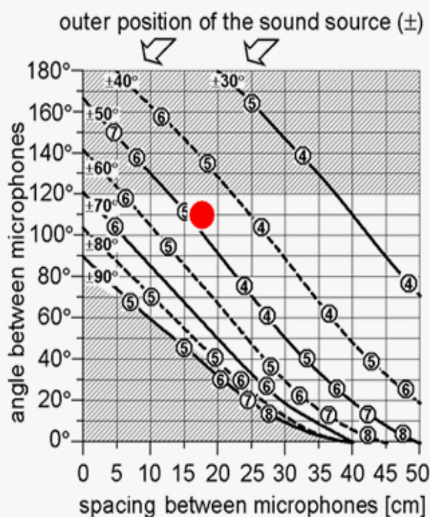
Fig. 20 The ORTF setup marked in a general diagram for cardioid microphones for XY setup.
