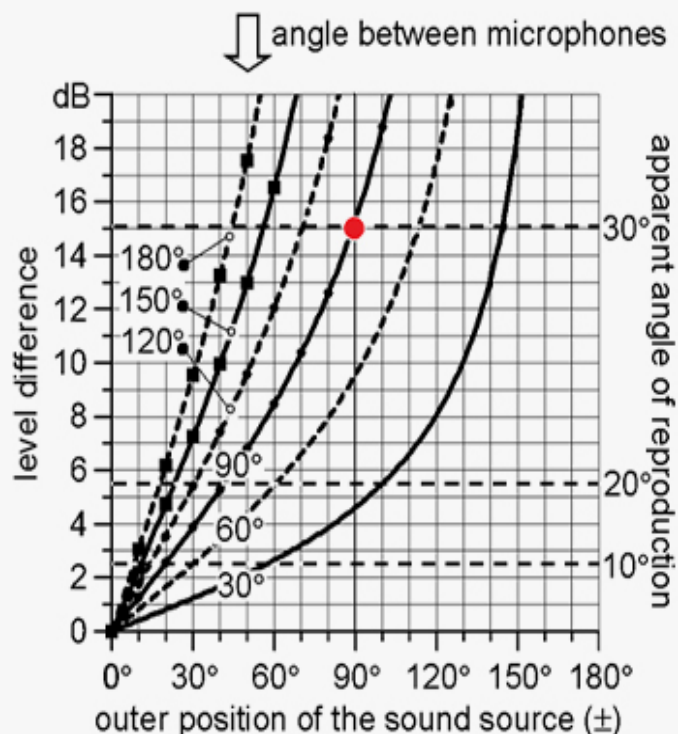
Fig. 10 Set of curves to determine the angle between two cardioid microphones for XY setup. The red dot marks the 90^\circ standard angling between the microphones.
