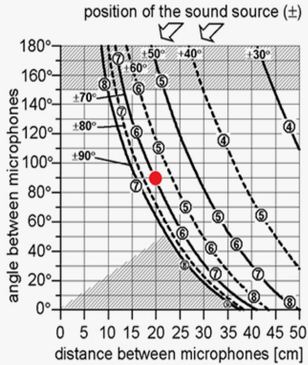
Fig. 16 Example, wide cardioid microphones: A recording of \pm 70^\circ can be achieved by spacing the wide cardioid microphones 20 cm and by a 90^\circ angling.
