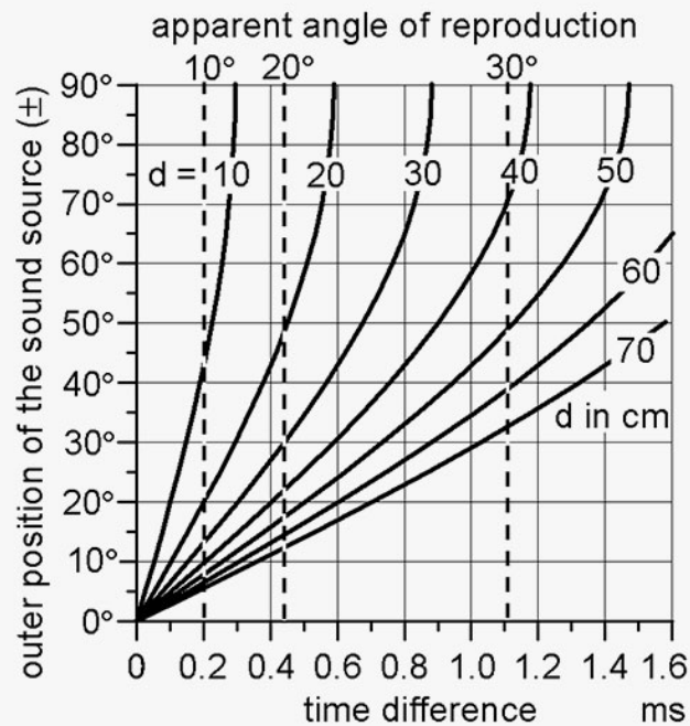
Fig. 6 Diagram to determine the distance between two omnidirectional microphones for the AB setup.
