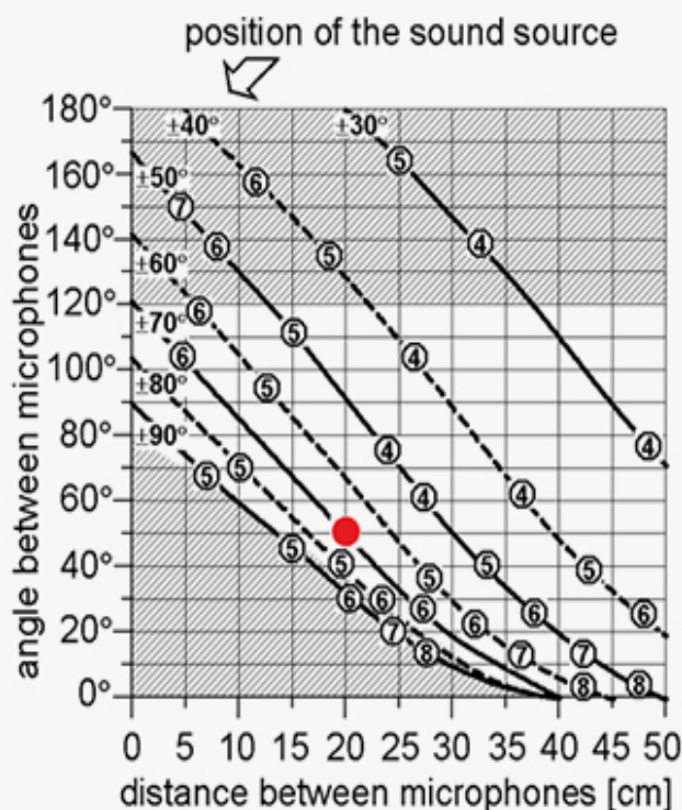
Fig. 15 Example, cardioid microphones: A recording angle of \pm 70^\circ can be achieved by spacing the cardioid microphones 20 cm (7.87 in) and by a 50^\circ angling. The angular distortion is marked by circles containing a number: The max deviation from the optimum angular position.
