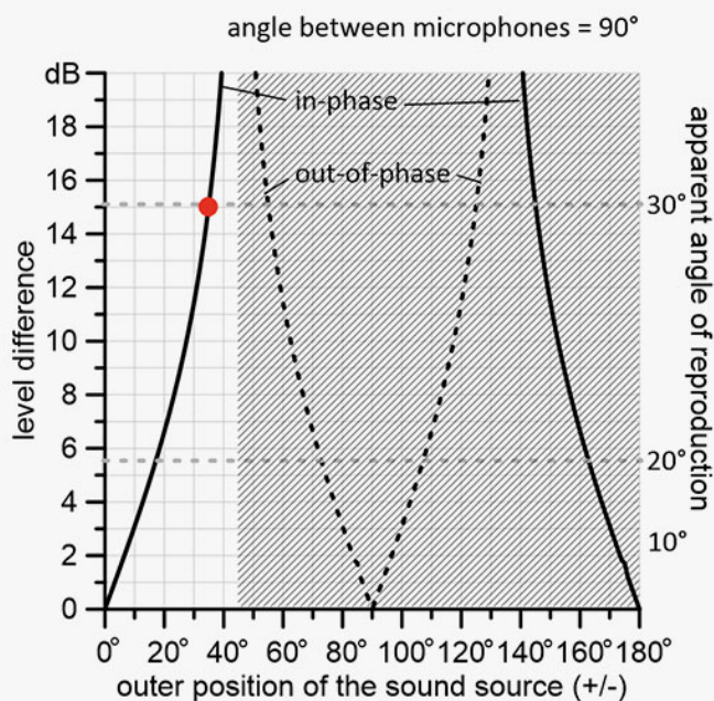
Fig. 12 Set of curves that show the level difference and phase between two bidirectional microphones angled \pm 45^\circ (Blumlein) dependent on the sound source position. The dashed lines in the grayed area indicate
