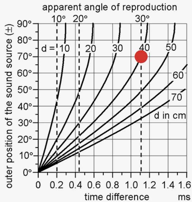
Fig. 7 The diagram to determine the distance between two omni microphones for the AB setup.
