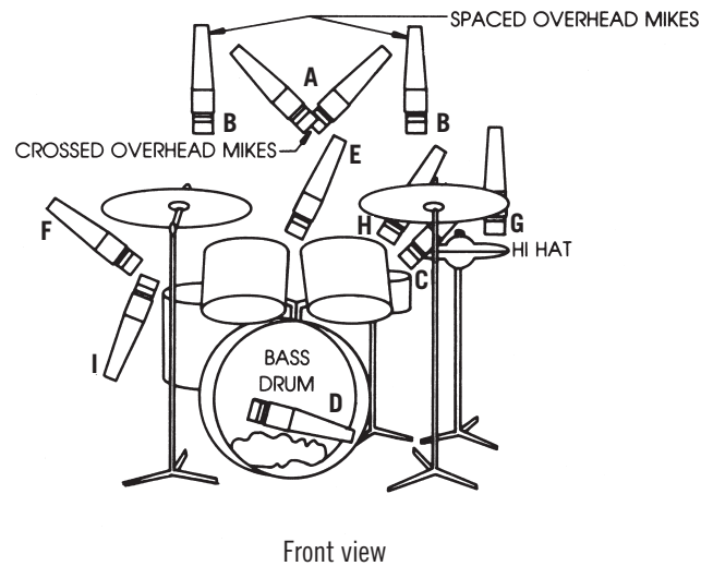
Image 10: Example of mic placement for hi-hats
