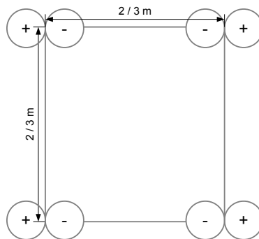
FIGURE 3 – Carré Hamasaki
