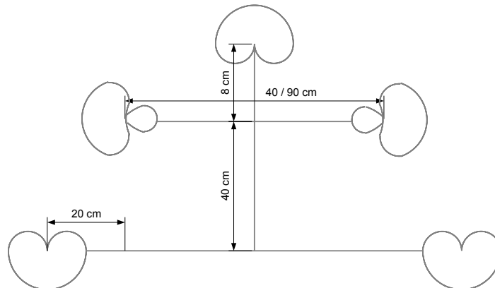
FIGURE 5 – OCT surround
