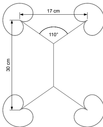
FIGURE 2 – Double ORTF
