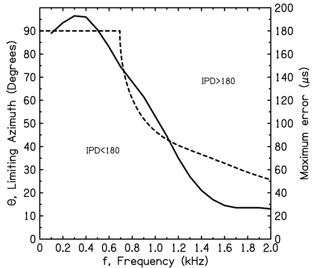
FIG. 2. Limits on ITDs in narrow-band signals caused by the \pi -limit. The dashed line shows the azimuth and frequency for which the IPD is 180° according to the spherical head model (the \pi -limit). The solid line (axis labels on the right) indicates the maximum error of the Woodworth formula within the boundaries of azimuth and frequency allowed by the \pi -limit.
